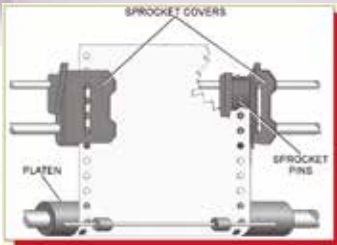
M355plus Continuous Print Module Pin-feed Tractor Mechanism
